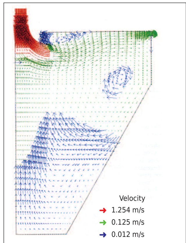
Flow velocities in the COANDA Grit Washer RoSF 4 (measured by TU Munich)
